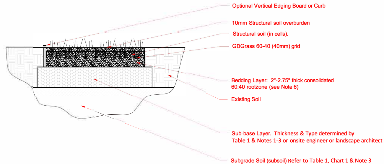
GDgrass™ 60-40 HDR :Grassed Surface: Typical Construction Profile Scale : N.T.S.
