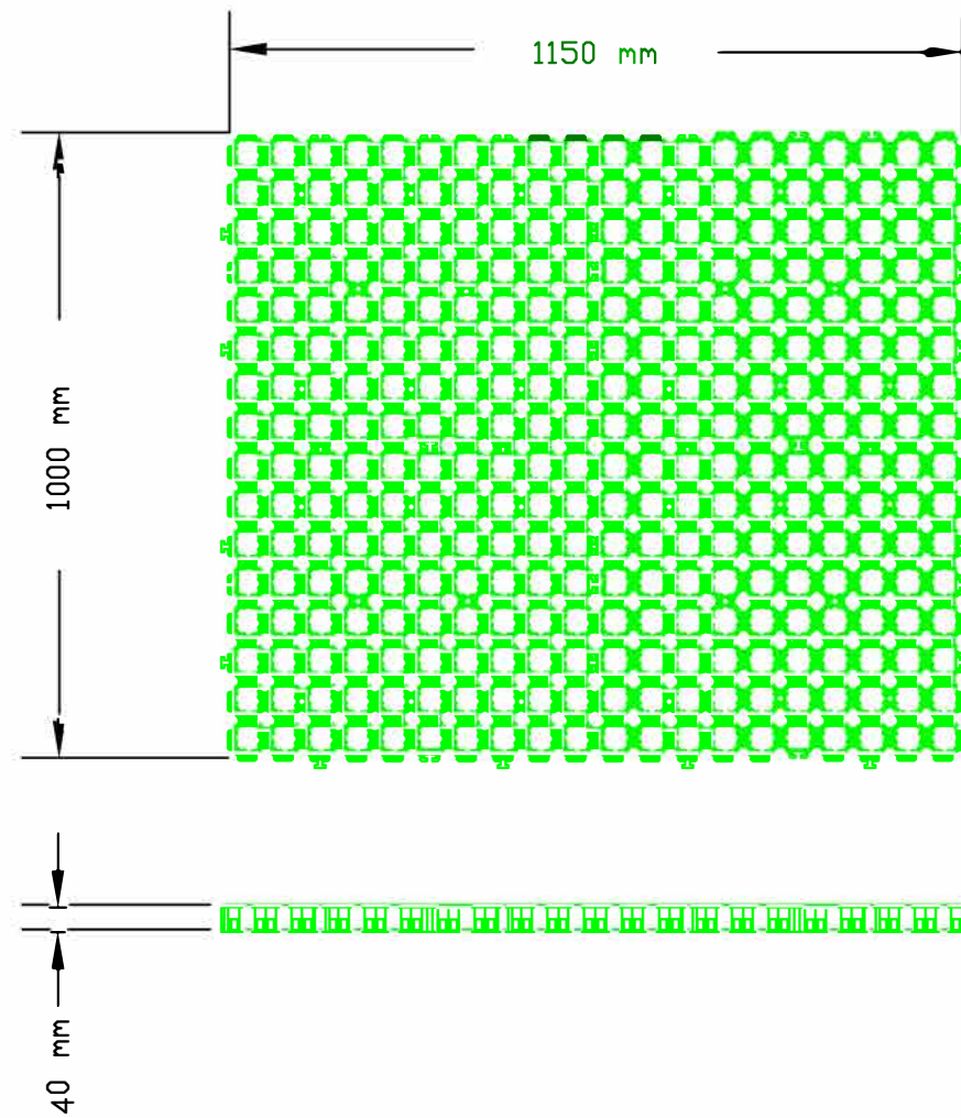
GDgrass™ 60-40 HDR :Grassed Surface Paving Grid Scale : N.T.S.
